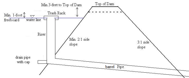
Riser should be 1.2 diameter of pipe Trash Rack should be 1.5 Riser diameter
